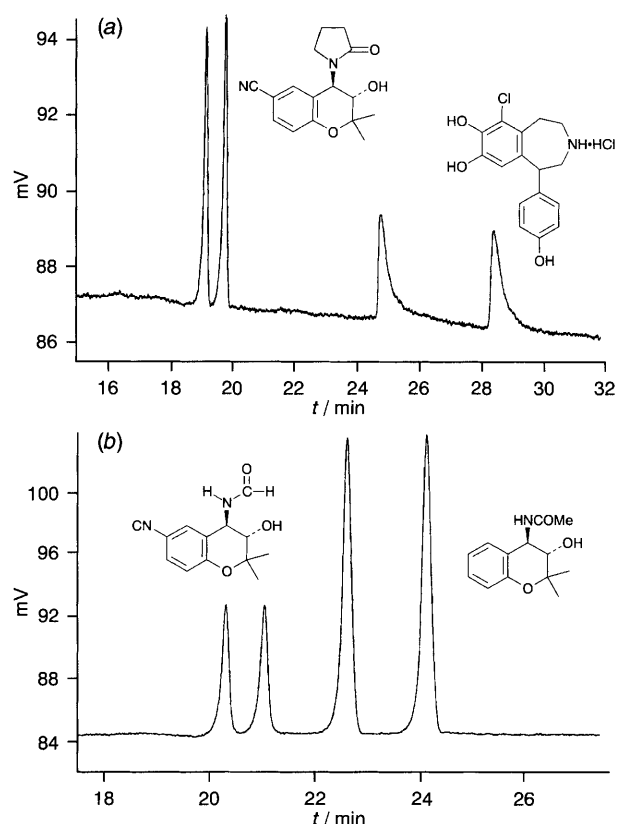
Fig. 2 Electropherograms of racemic mixtures of (a) cromakalin and fenoldopam and (b) two cromakalin-related molecules using 1a (25 mmol dm -3 ) in the separation buffer. Conditions : Fused-silica capillary, 670 mm × 50 μm; 50 mmol dm -3 borate–25 mmol dm -3 phosphate buffer, pH 7.0; 20 °C; voltage, 12.5 kV; sample, 3s pressure injection of a solution ca. 1 × 10 -4 mol dm -3 in water; detection wavelength, 254 nm.
